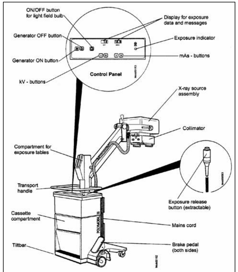
Polymobil Operation Schematics
